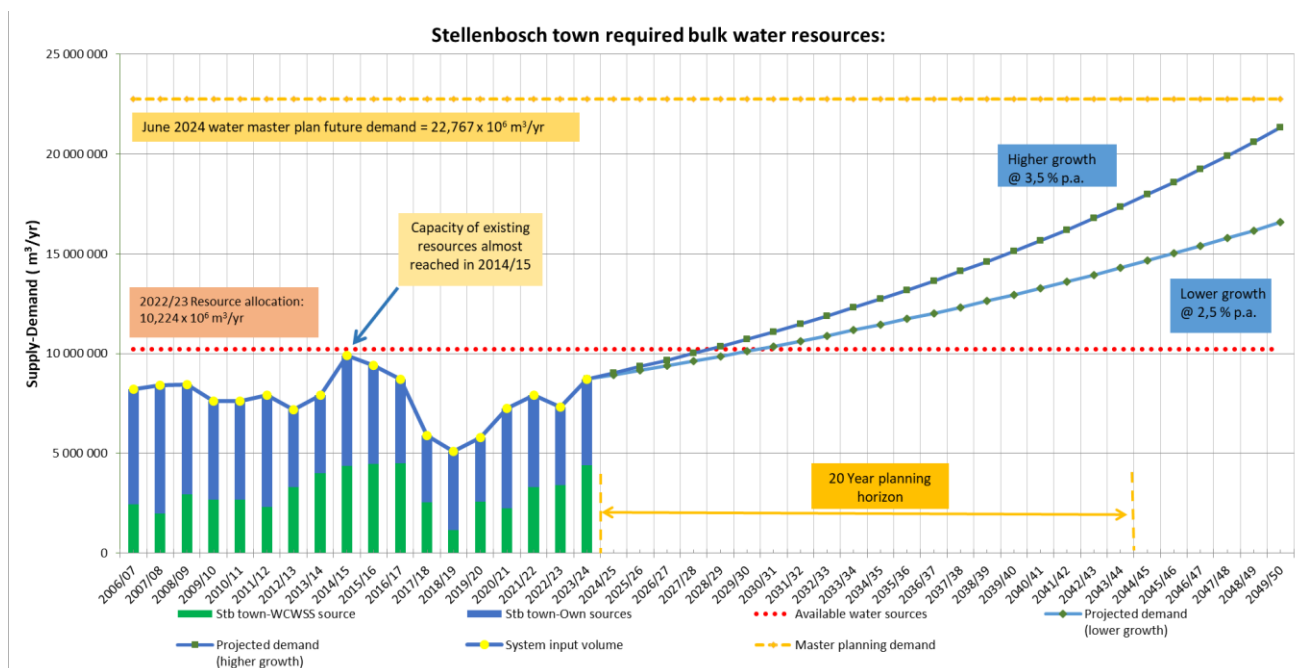
Figure 49: Bulk Water Resources
