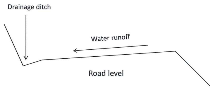
Figure 19: Road surface slope with a drainage ditch
