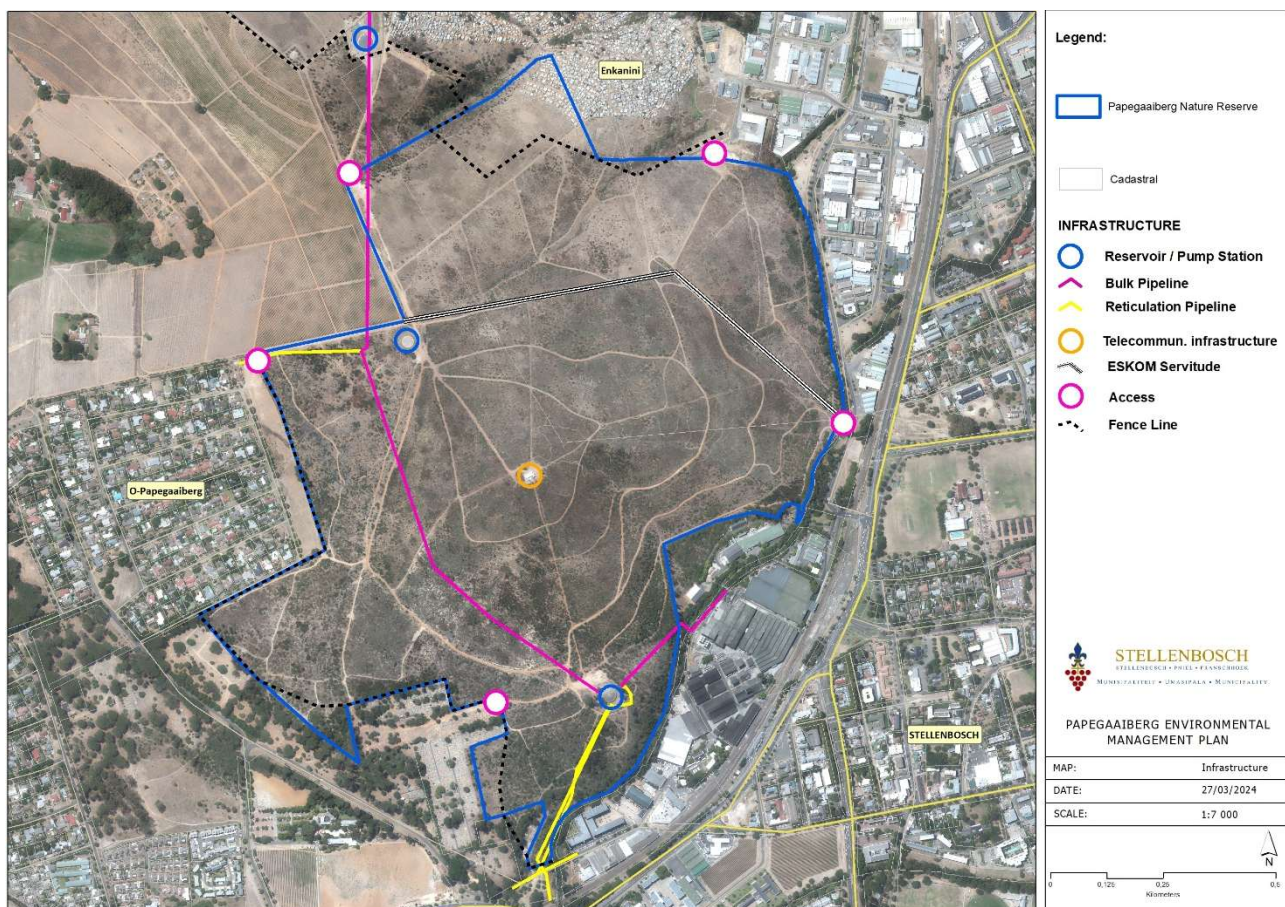
Figure 4: Cadastral boundaries and infrastructure of Papegaaiberg NR.
