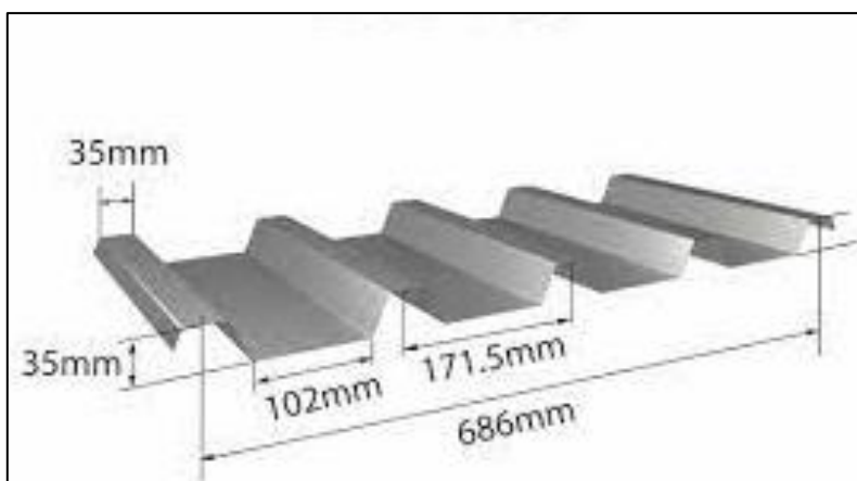
Figure 2: IBR roof sheet
