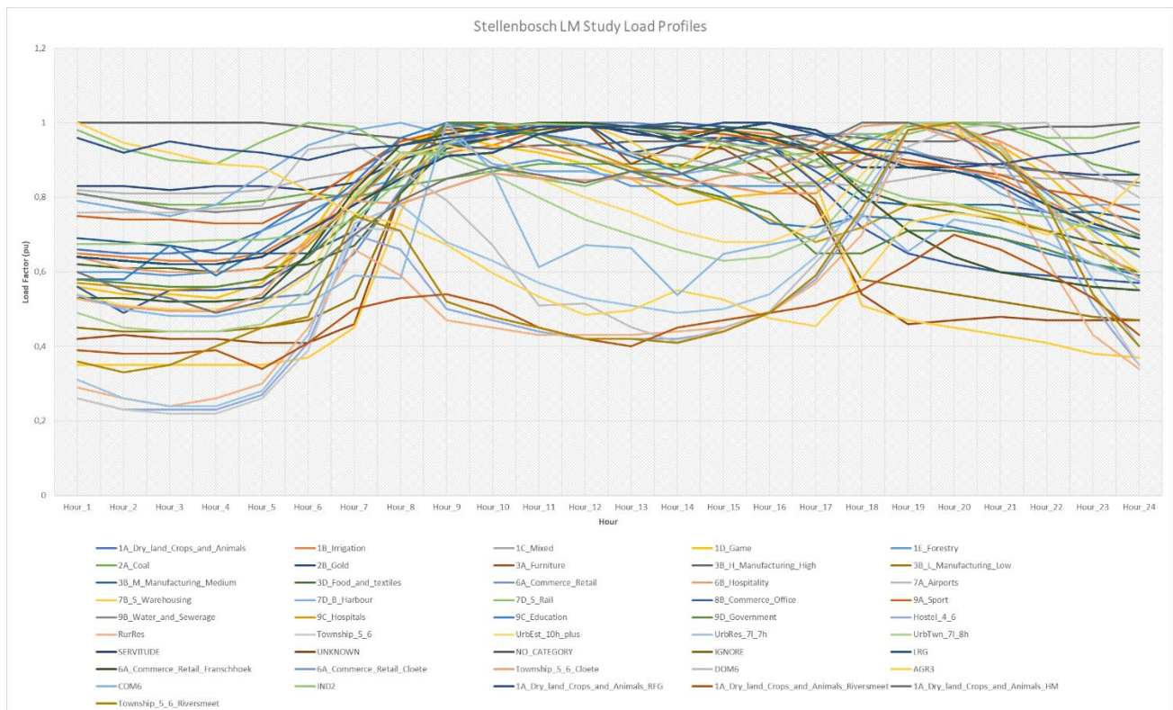
Figure 5-11: Standard and Stellenbosch-customized Load Profile Curves
