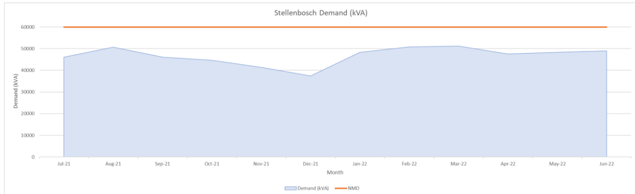
Figure 4-5: Stellenbosch Main monthly demand trend
