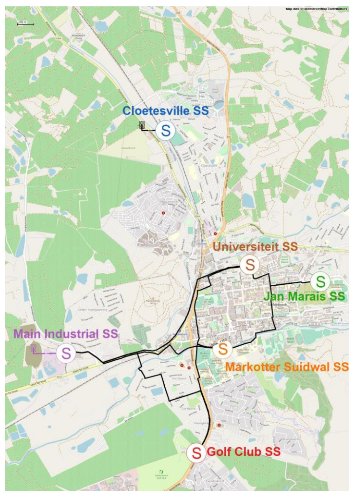
Figure 7-1: Stellenbosh Geospatial 66kV Network
