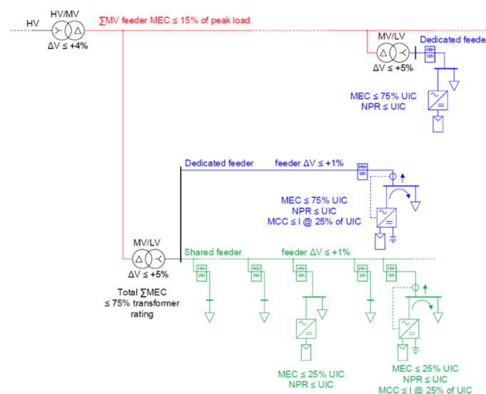
Figure 8-4: NRS 097-2-3 Simplified Connection Criteria [10]
