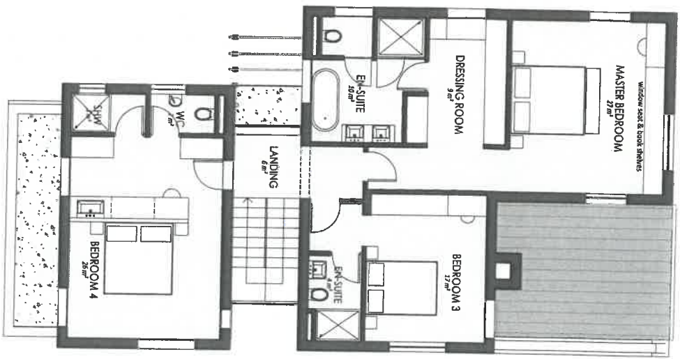
FIRST FLOOR PLAN Scale 1 : 100
