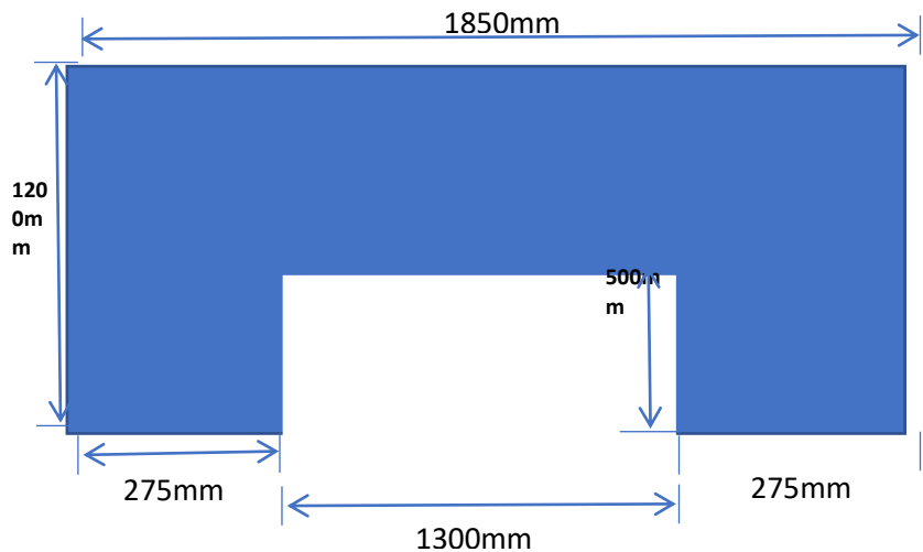
4 way concrete plinth
