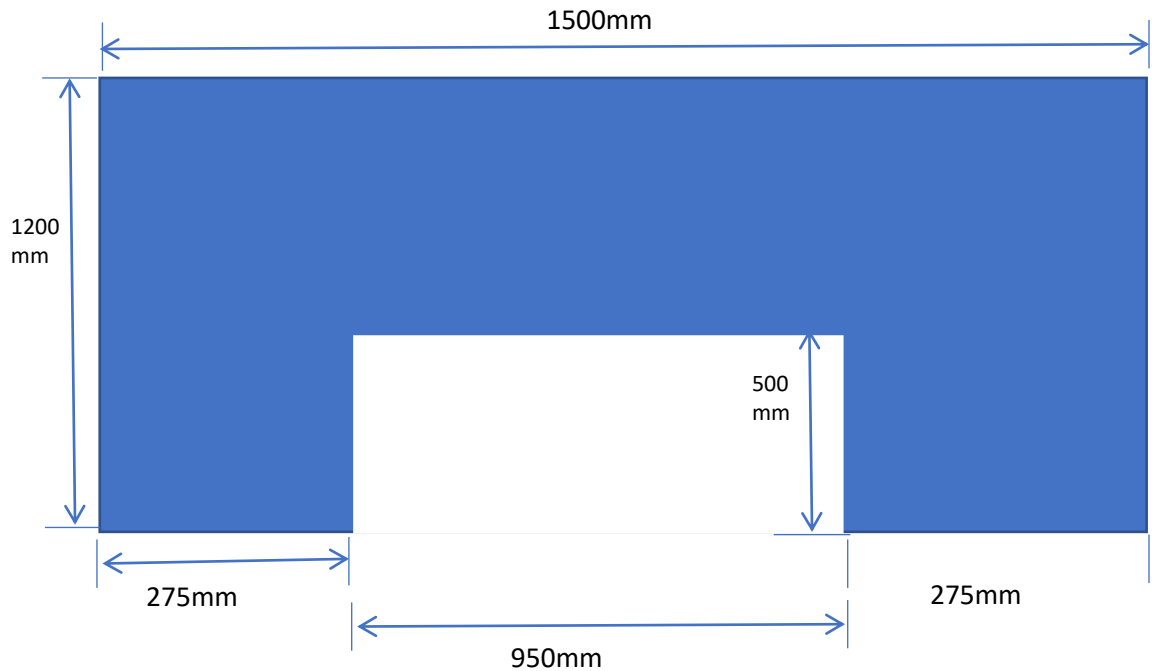
3 way concrete plinth
