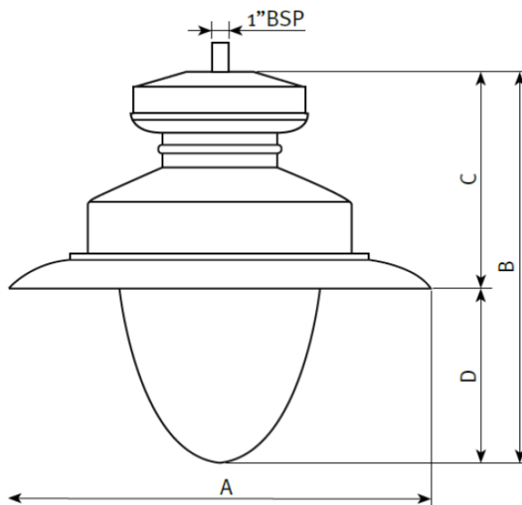
Illustration of the decorative bell shaped LED
