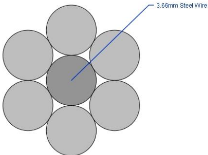
Figure 1: Illustration of ACSR mink overhead ungreaed conductor construction
