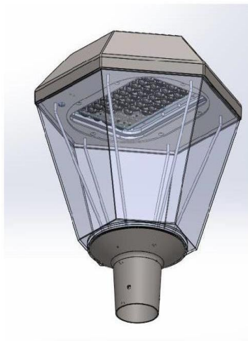
LED Luminaire Complete
