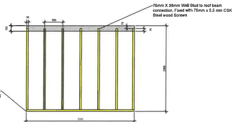
Typical Wall Frame Section
