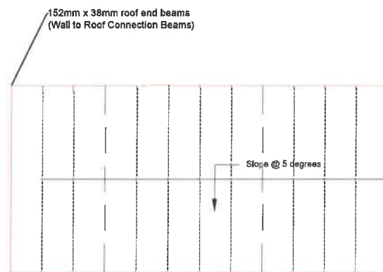
Roof Layout Plan
