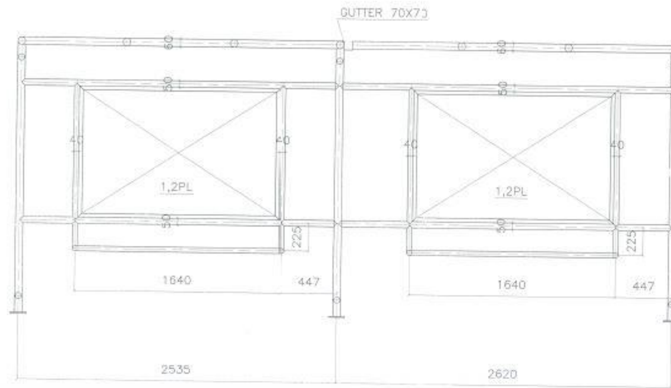
FRONT ELEV
