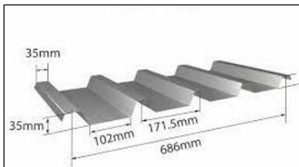
Profile of 0.7mm IBR roof sheet
