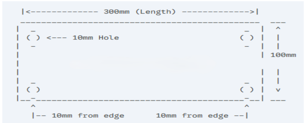
Figure 2: Numbering Plate Template
