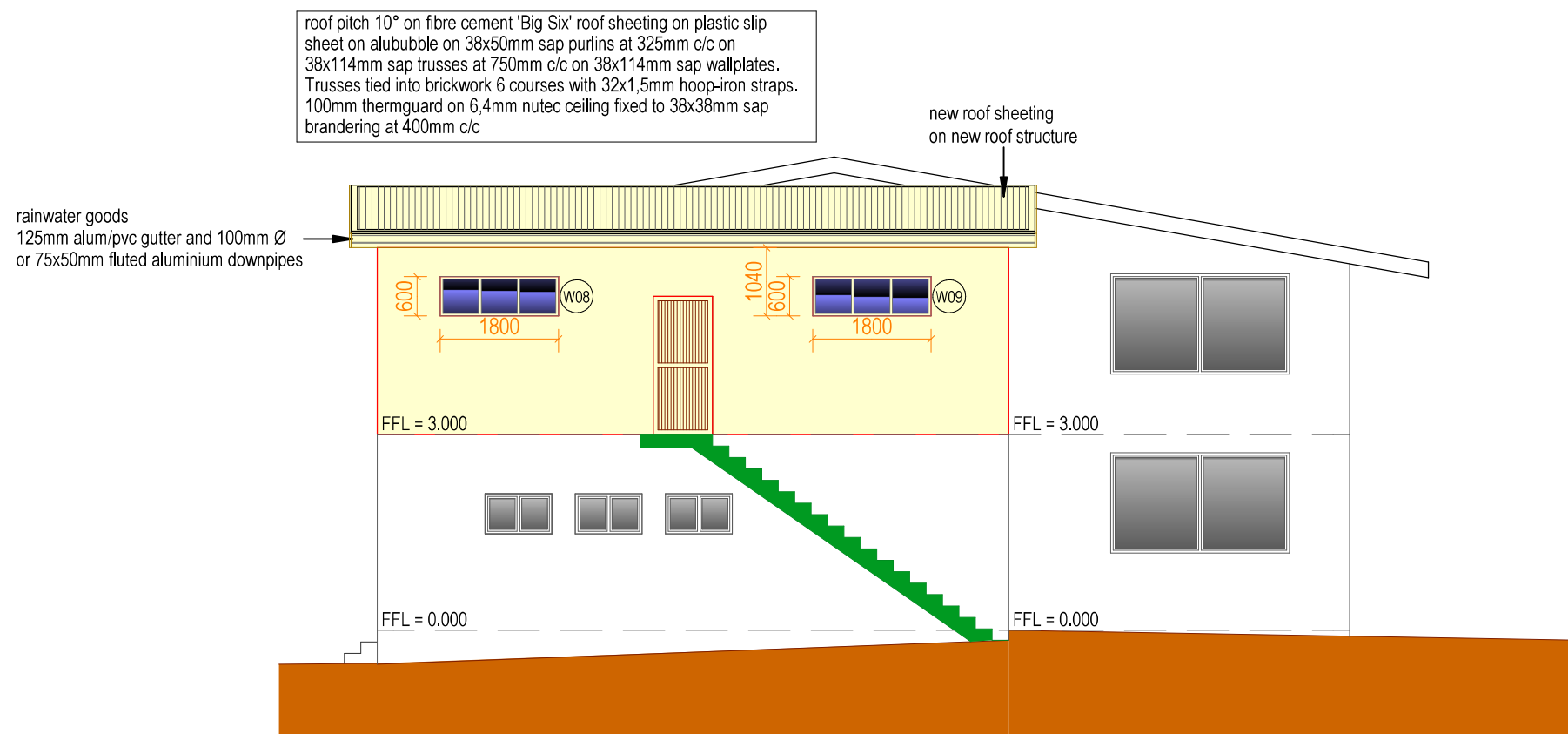
South Elevation 1:100
