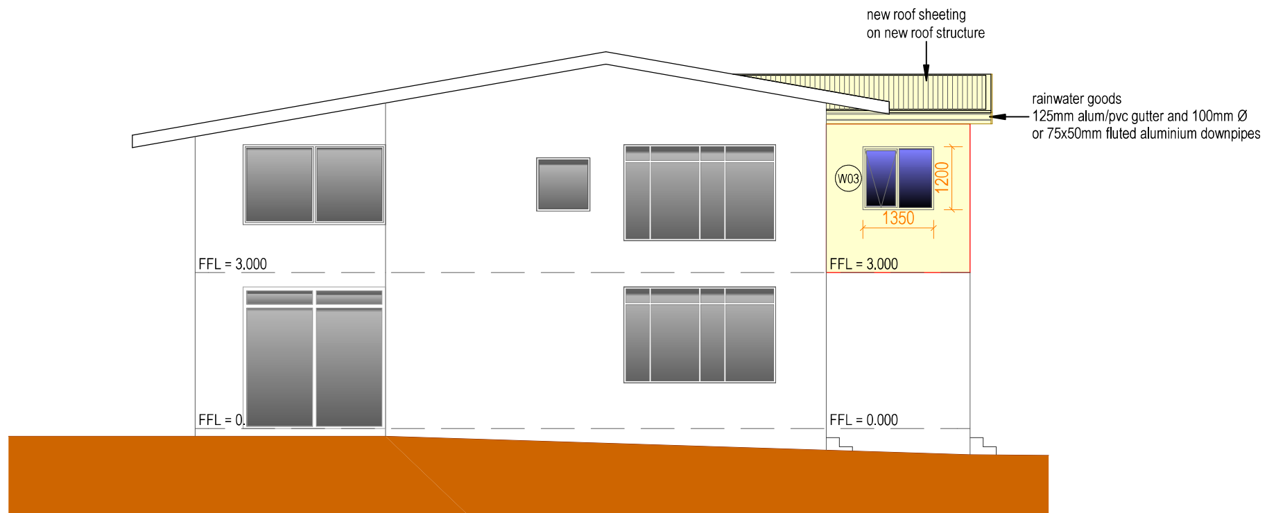
North Elevation 1:100
