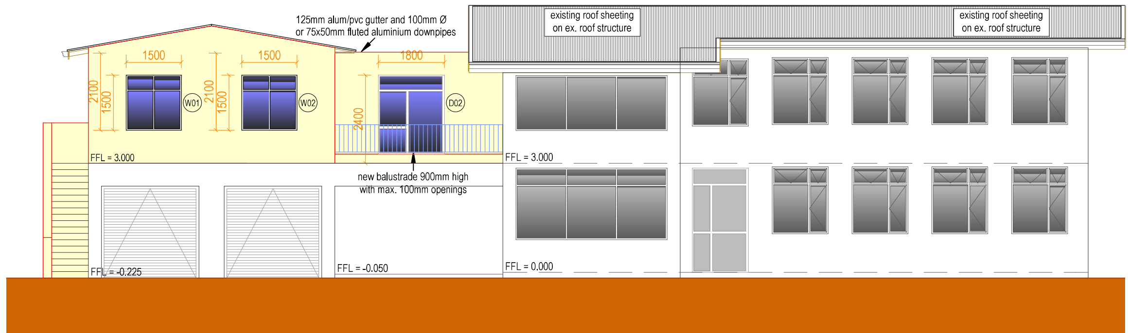
East Elevation 1:100
