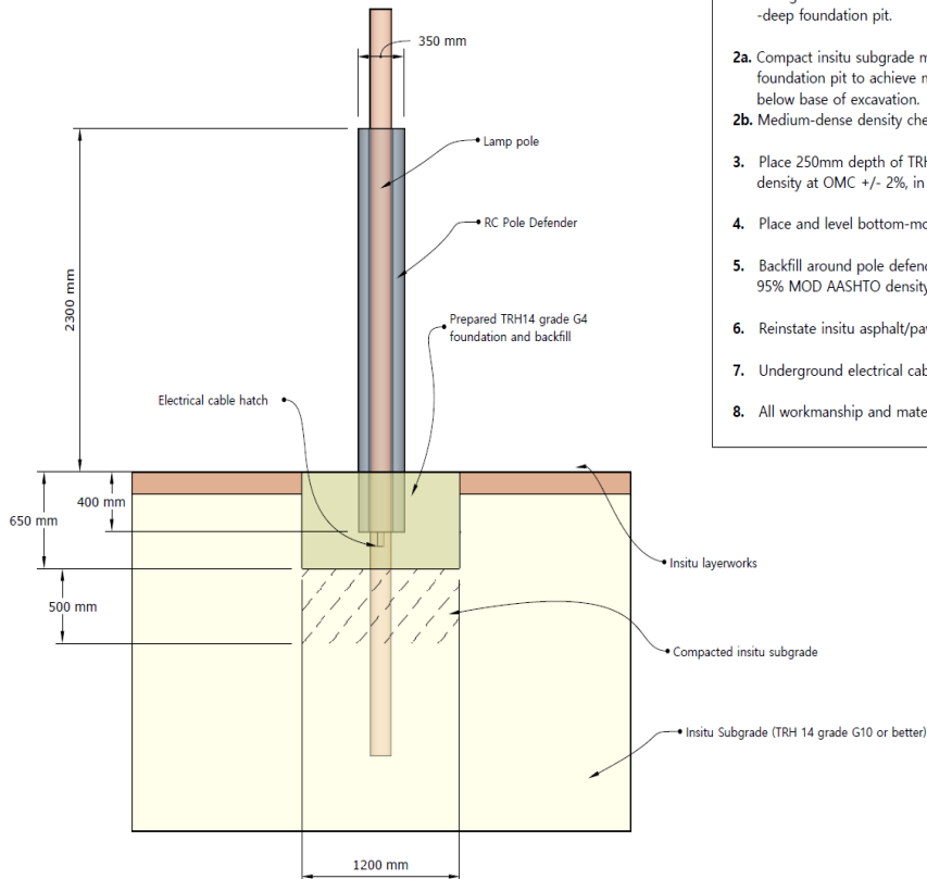
POLE DEFENDER FOUNDATION SECTIONAL VIEW
