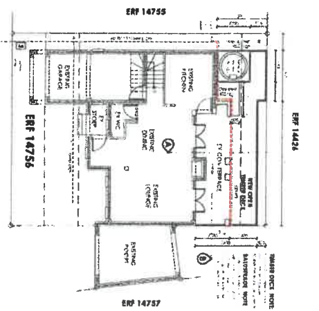
GROUND FLOOR LAYOUT SCALE 1:100
