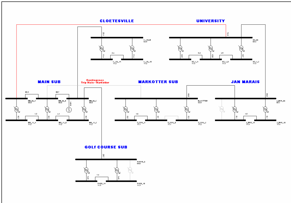
Figure 12: Main – Markotter Contingency, 2025 Load
