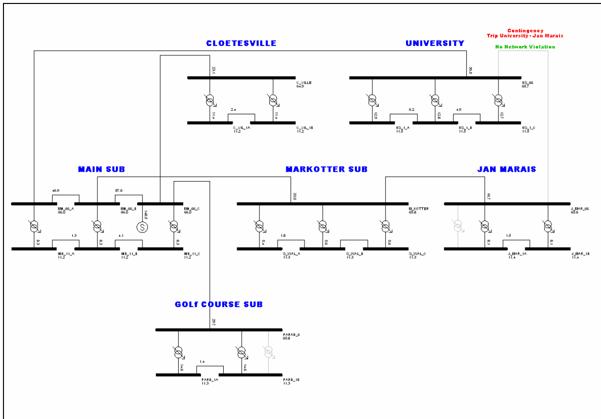
Figure 20: University – Jan Marais Contingency, 2025 Load
