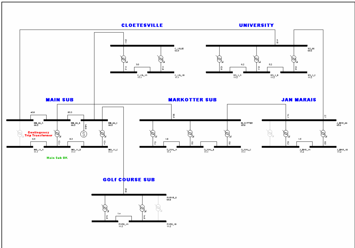
Figure 6: Main – Transformer Contingency, 2025 Load
