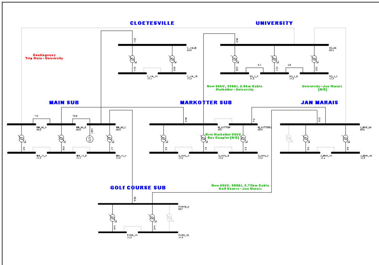
Figure 17: Main – University Solution 2, 2025 Load
