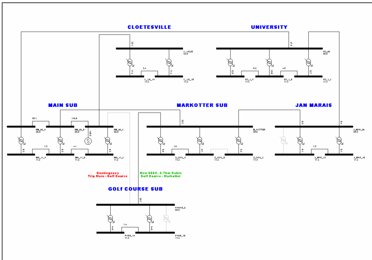
Figure 10: Main – Golf Course Contingency Solution 1, 2025 Load
