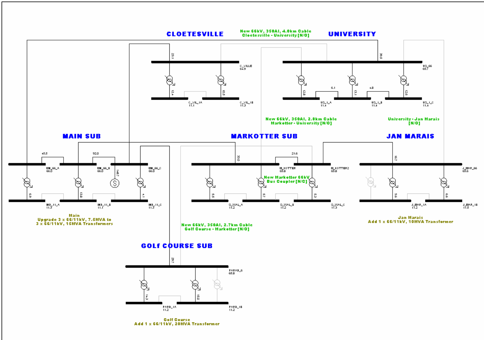
Figure 21: 66kV Network Recommendations, 2025 Load
