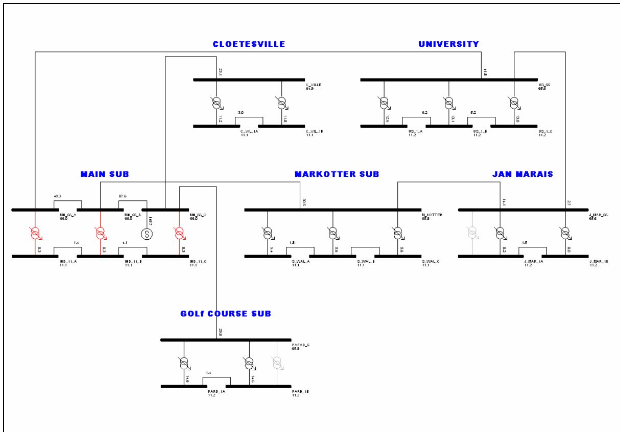
Figure 4: Main – Transformer Existing, 2025 Load
