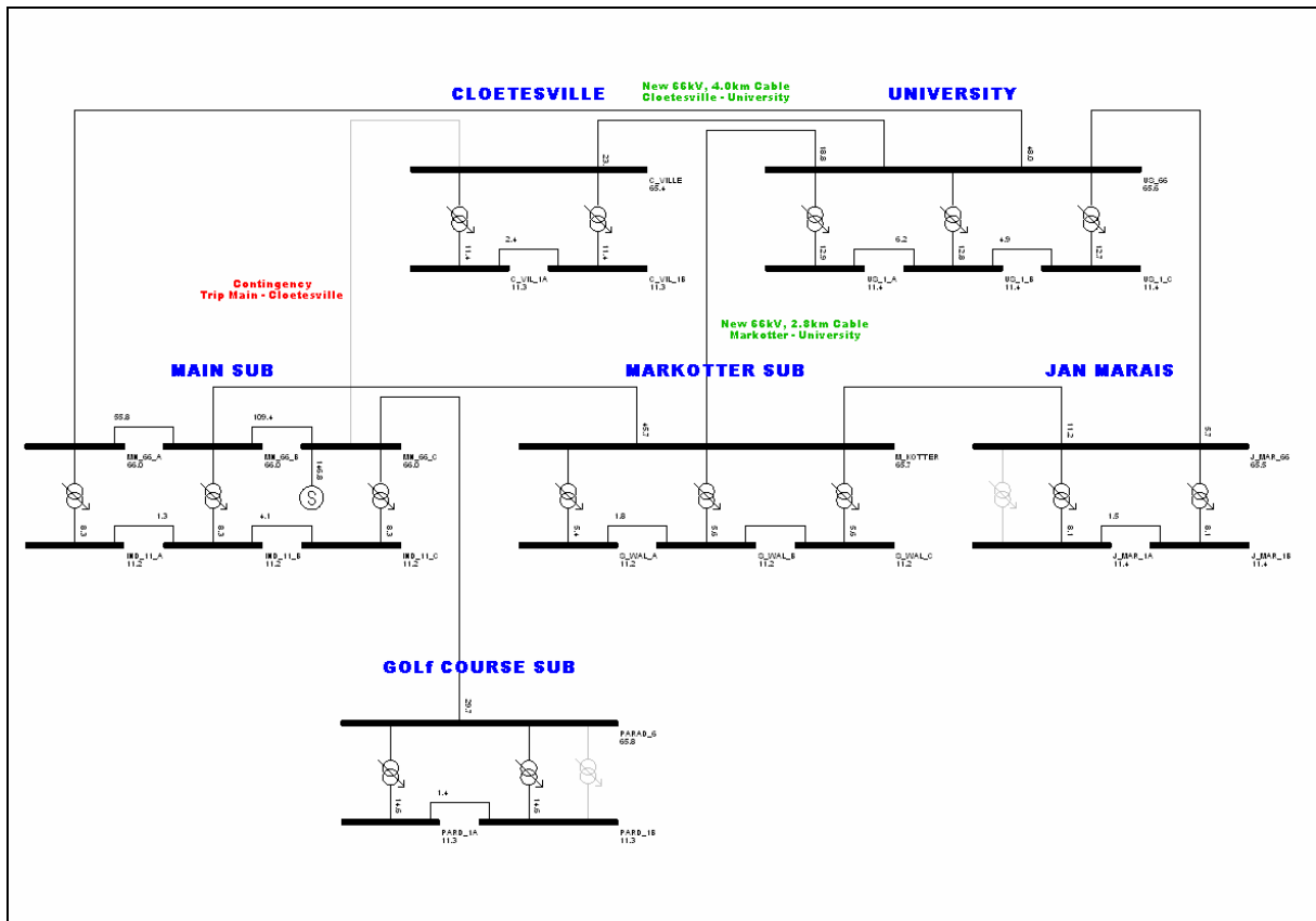
Figure 9: Main – Cloetesville Contingency, 2025 Load
