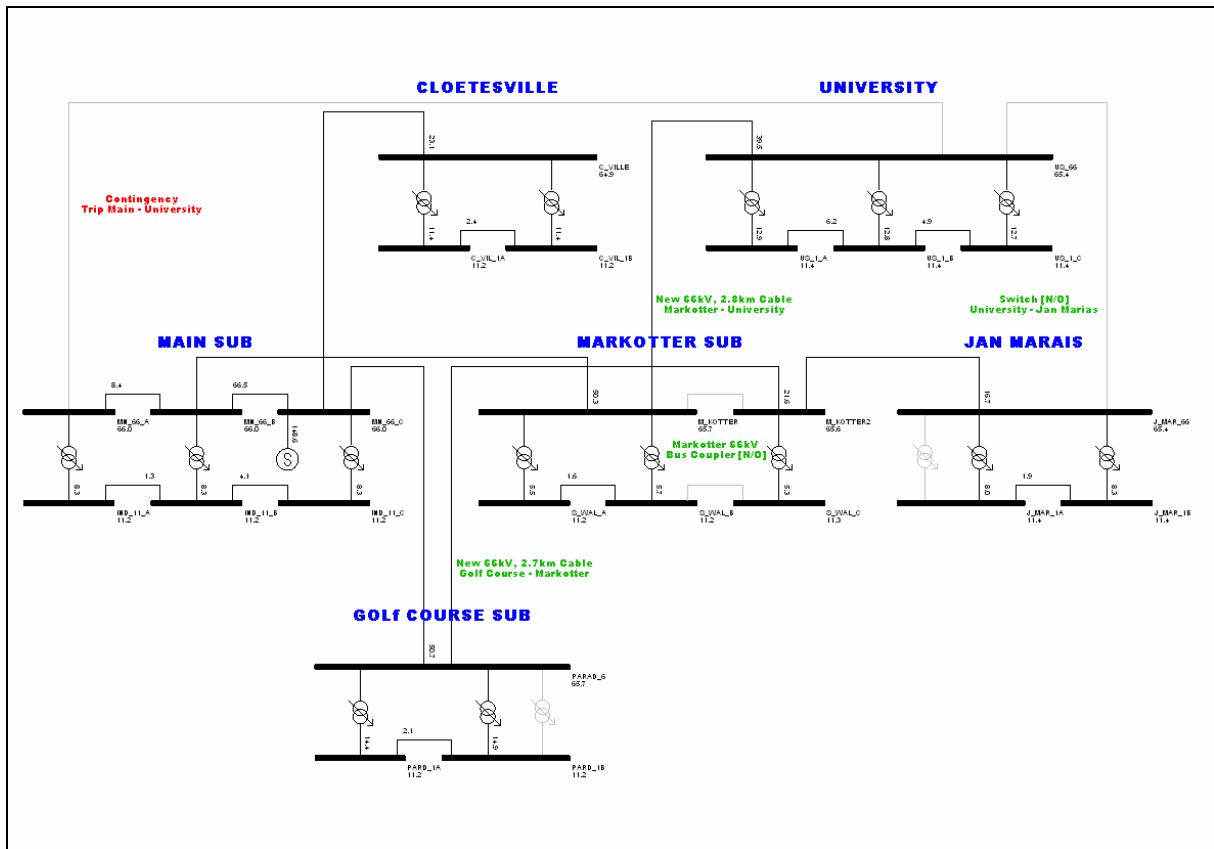
Figure 16: Main – University Solution 1, 2025 Load
