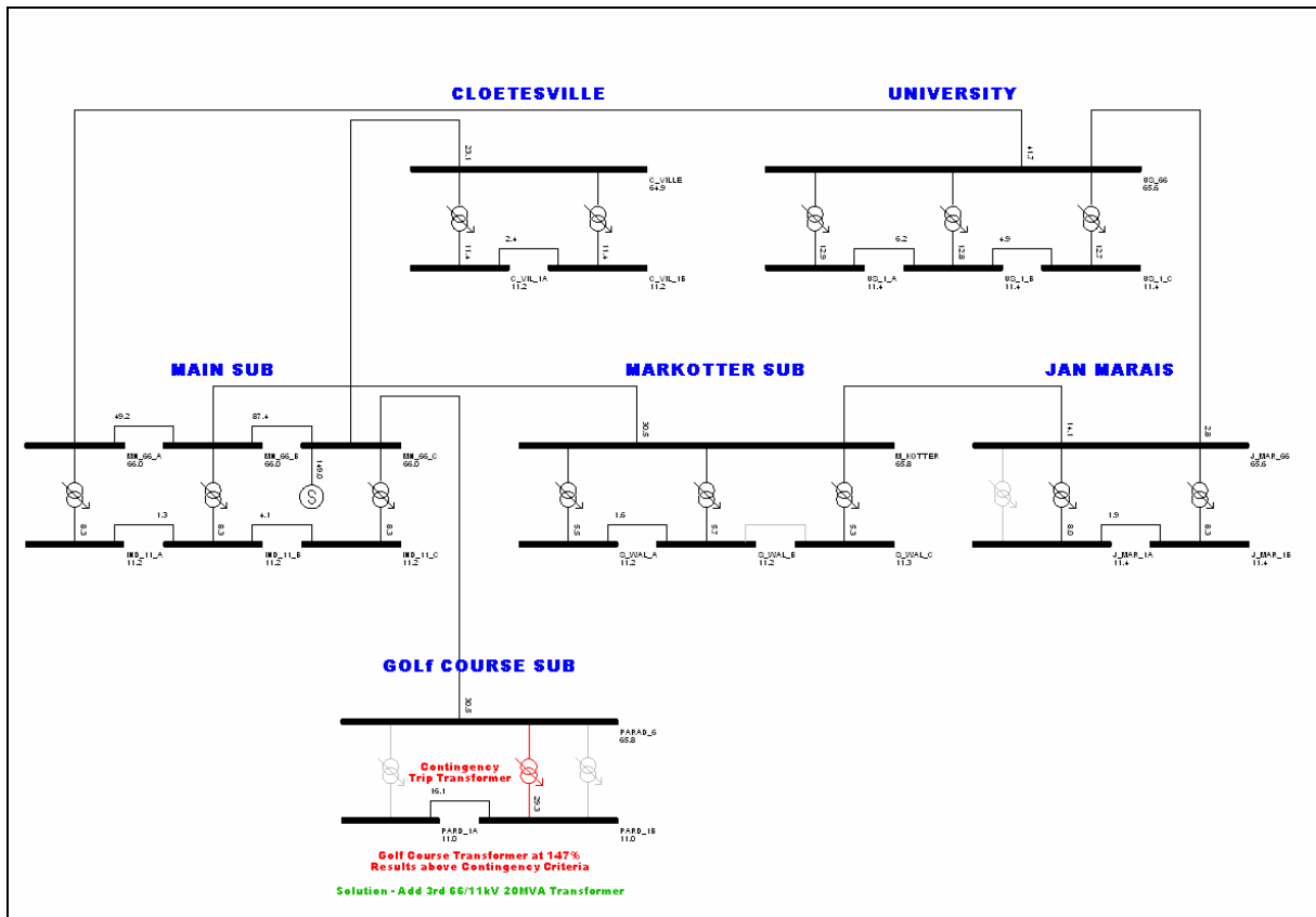
Figure 2: Golf Course – Transformer Contingency, 2025 Load
