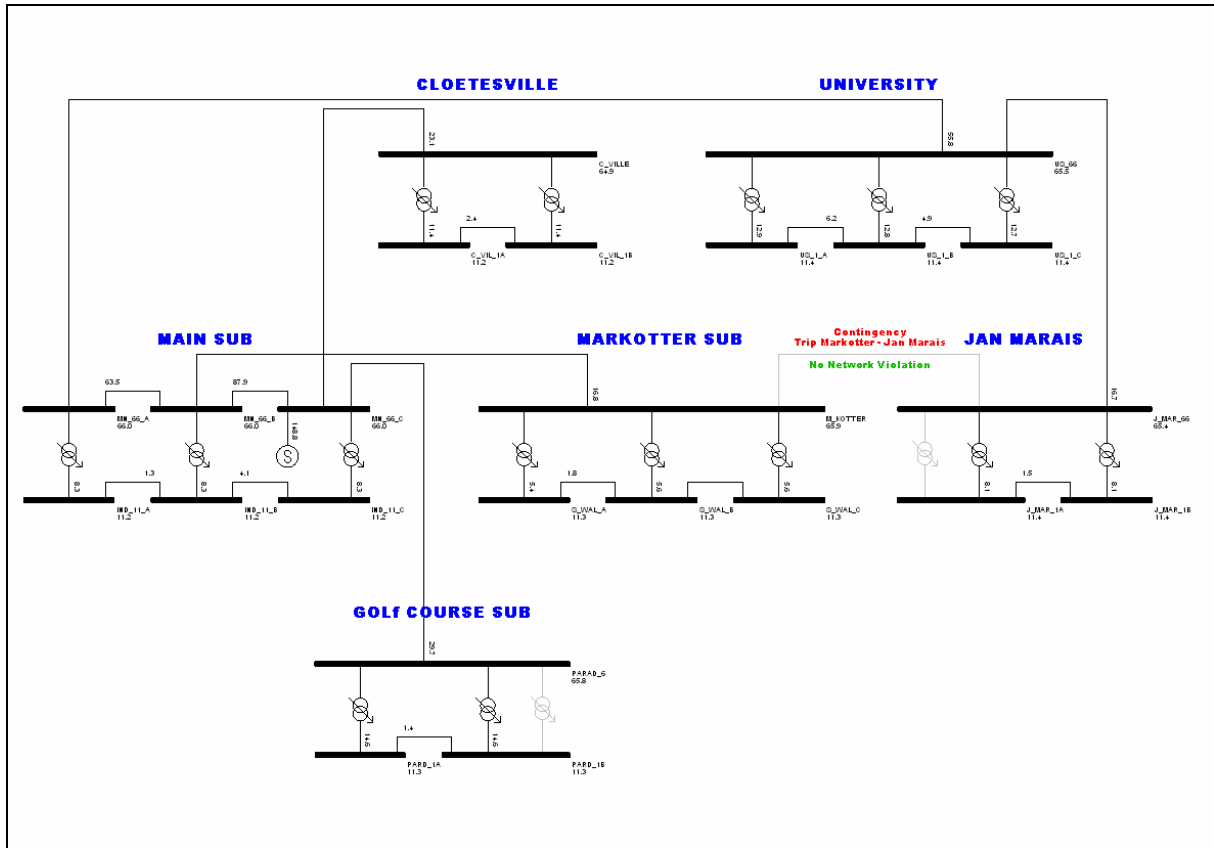
Figure 19: Markotter – Jan Marais Contingency, 2025 Load
