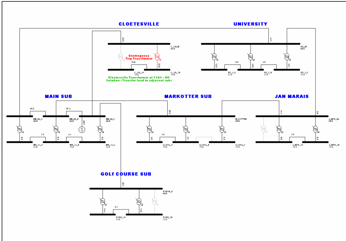
Figure 1: Cloetesville – Transformer Contingency, 2025 Load
