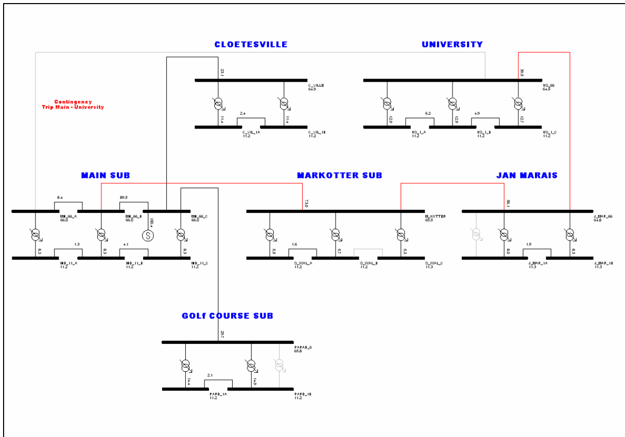
Figure 15: Main – University Contingency, 2025 Load
