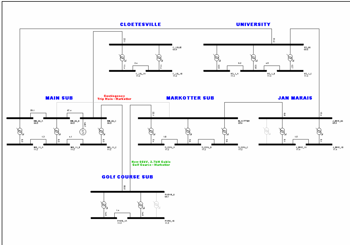
Figure 13: Main – Markotter Solution 1, 2025 Load
