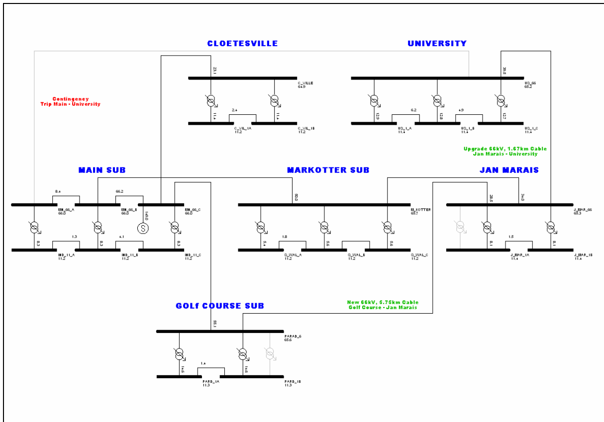
Figure 18: Main – University Solution 3, 2025 Load
