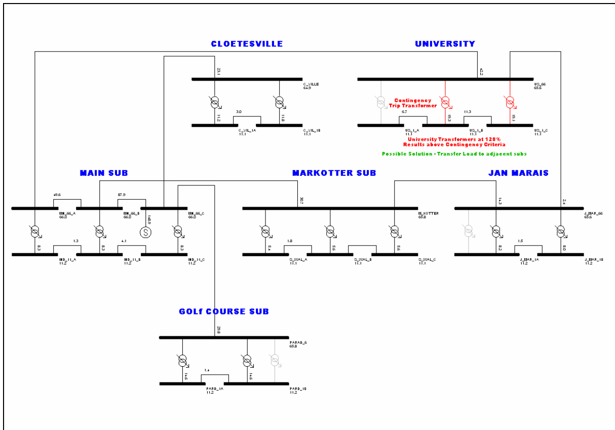
Figure 8: University – Transformer Contingency, 2025 Load
