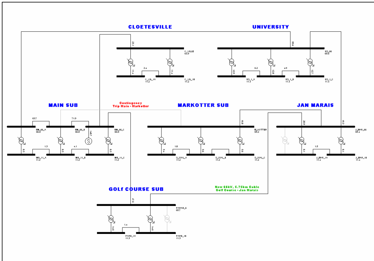
Figure 14: Main – Markotter Solution 2, 2025 Load
