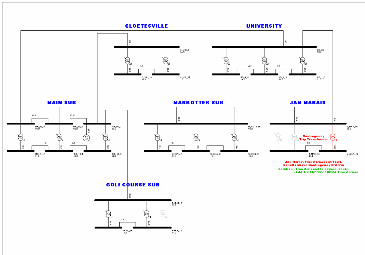
Figure 3: Jan Marais – Transformer Contingency, 2025 Load
