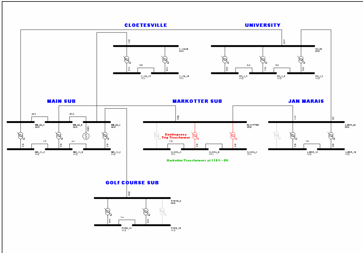
Figure 7: Markotter – Transformer Contingency, 2025 Load
